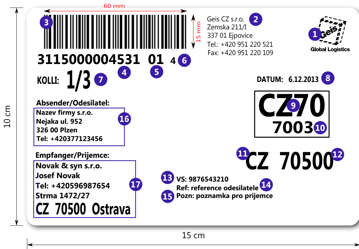
Figure 3: Label layout
